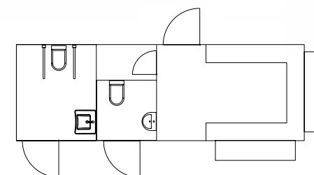
4 WC Quiosque 2400x7200mm WC Quiosco 2400x7200mm
